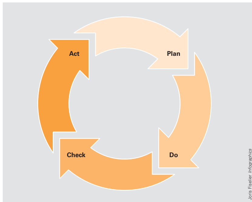
Figuur 5 Plan-do-check-act-cyclus
