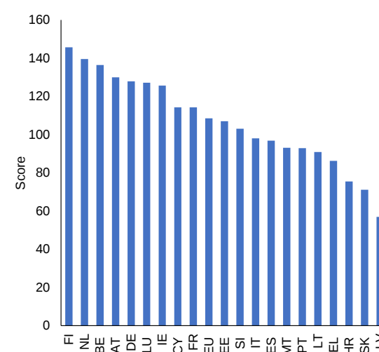
Graph 5.8: Innovation Index
