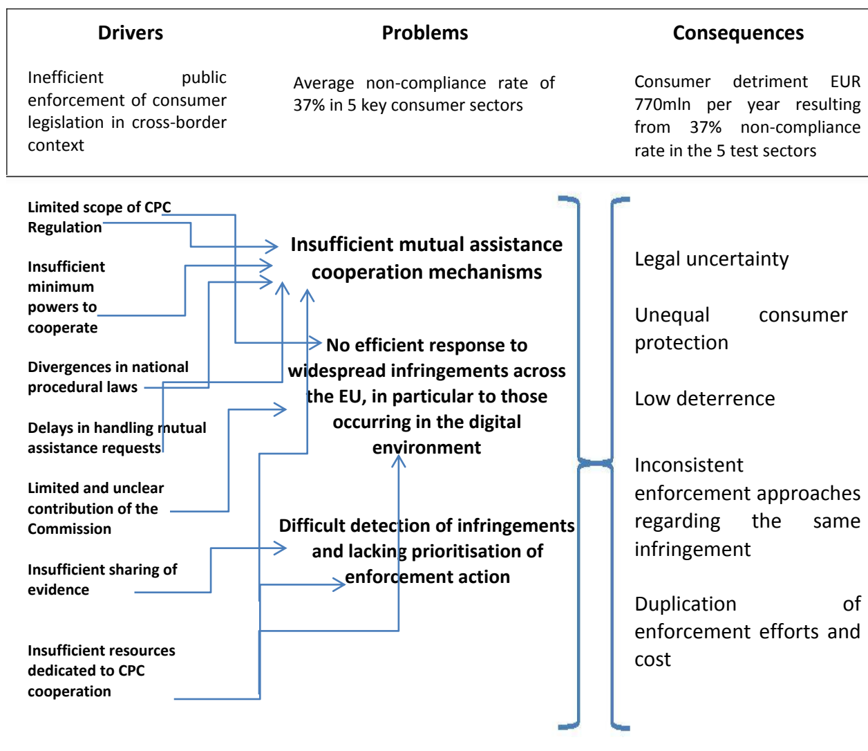
Figure 1: Problem Tree
