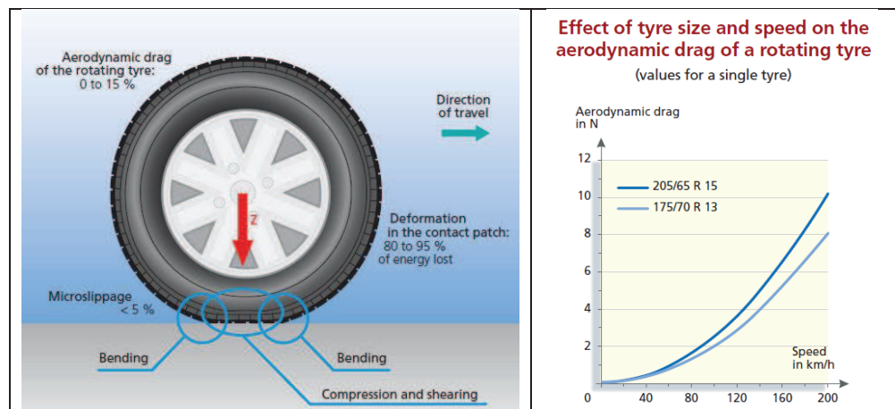
Figure 3.12: The 3 main causes of rolling resistance [16].
