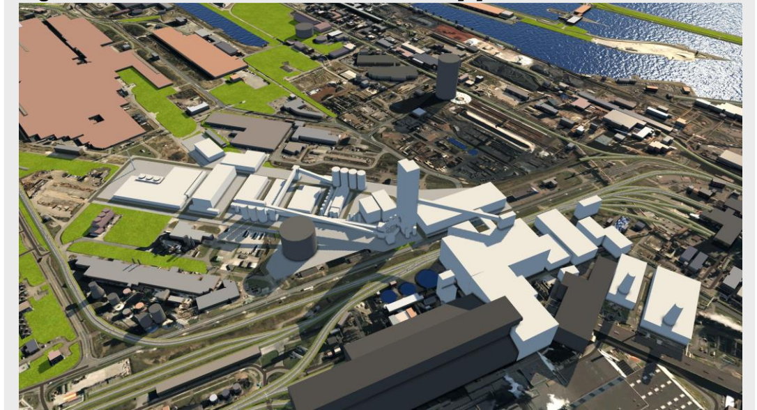
Figure 16. 3D model Green Steel Phase 1 [6]
