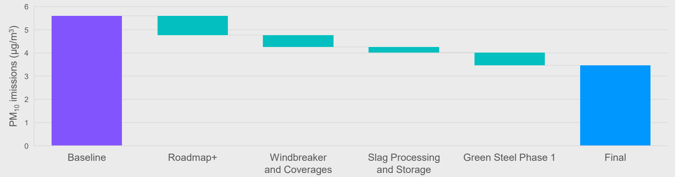
Figure 11. TSN's predicted PM 10 immission contribution reductions in WaZ [6]
