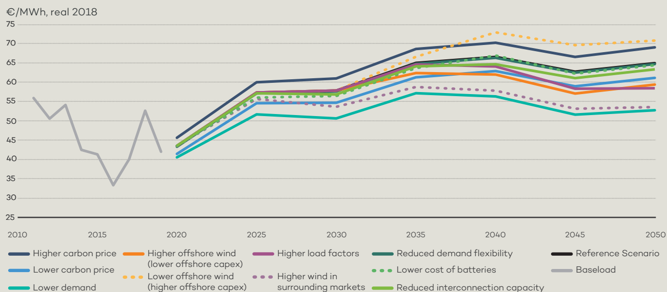
FIGURE 28 – WHOLESALE ELECTRICITY (DAY-AHEAD) PRICES FOR THE NETHERLANDS, (€/MWh)
