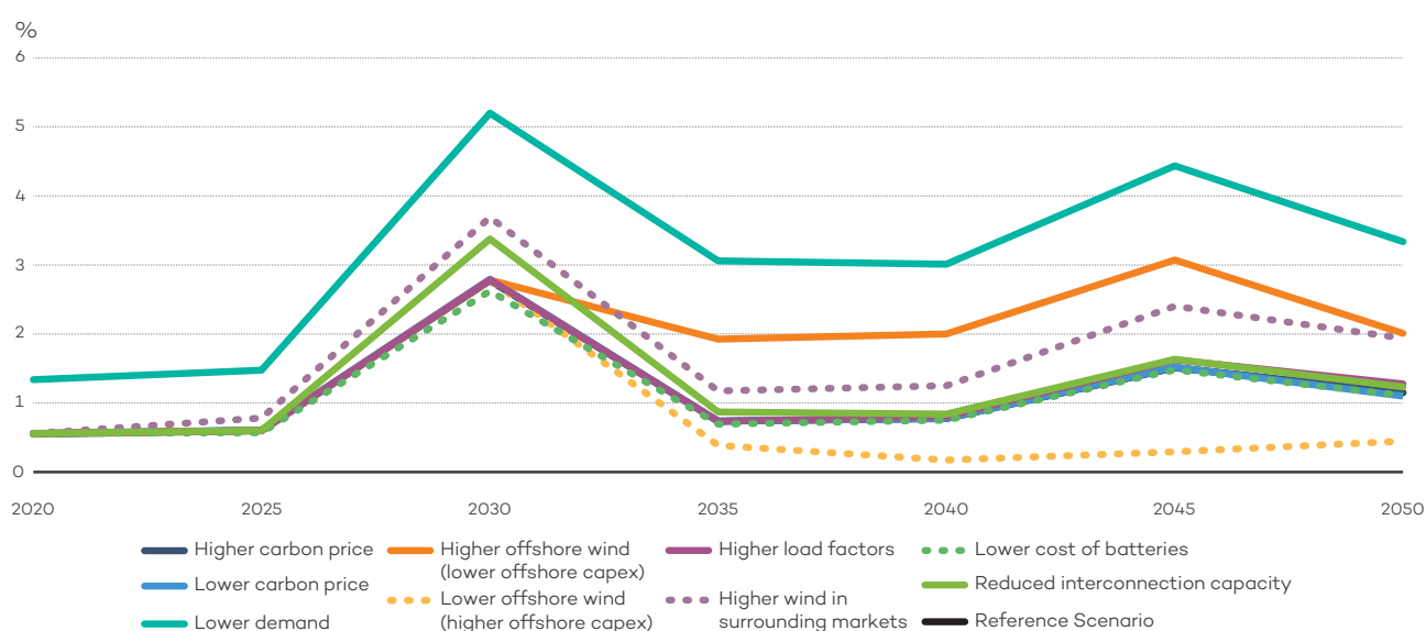
FIGURE 23 – LEVELS OF WIND CURTAILMENT (AS % OF GENERATION) FOR SENSITIVITIES
